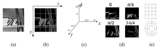
GLOH
