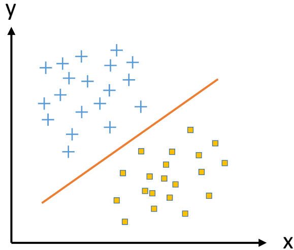
Linearly inseparable
