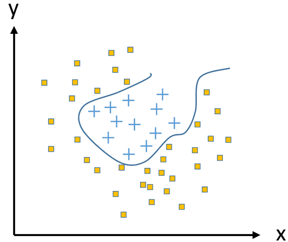
Non-linearly inseparable
